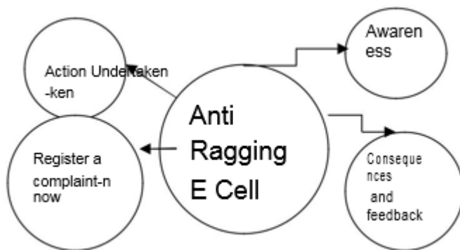
Fig 1: Architecture Diagram
